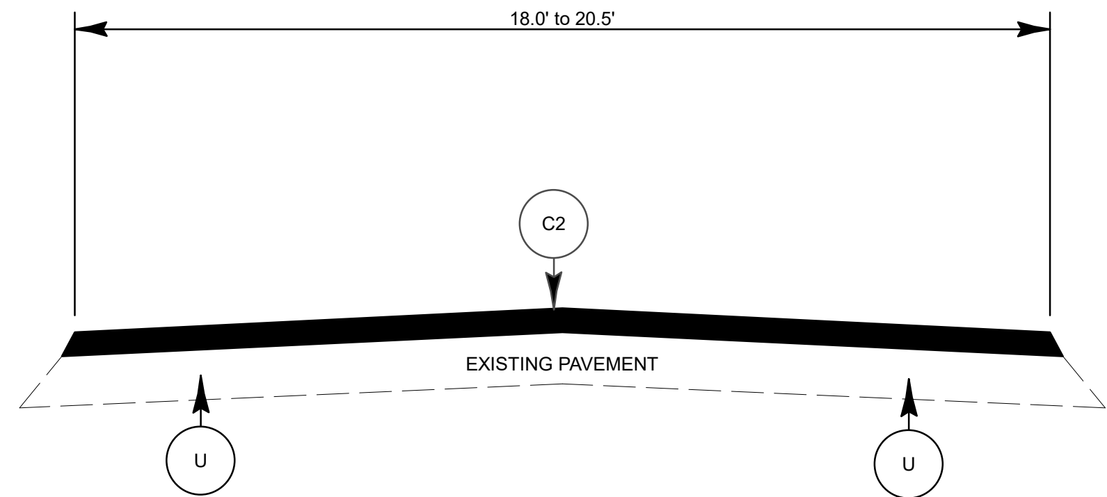
TYPICAL SECTION NO. 3
